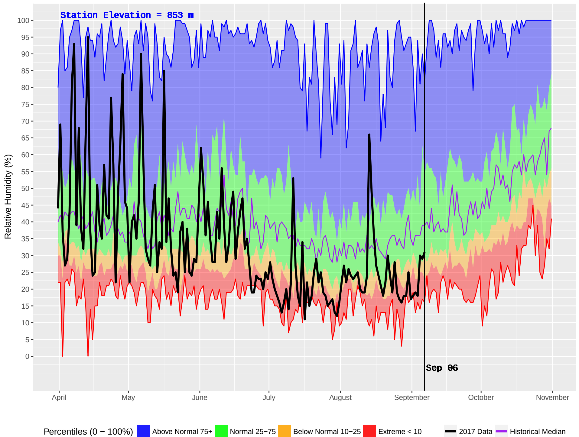
JOHNSON LAKE (419) : Historical (1986–2016) and Current (2017) Noon Relative Humidity
