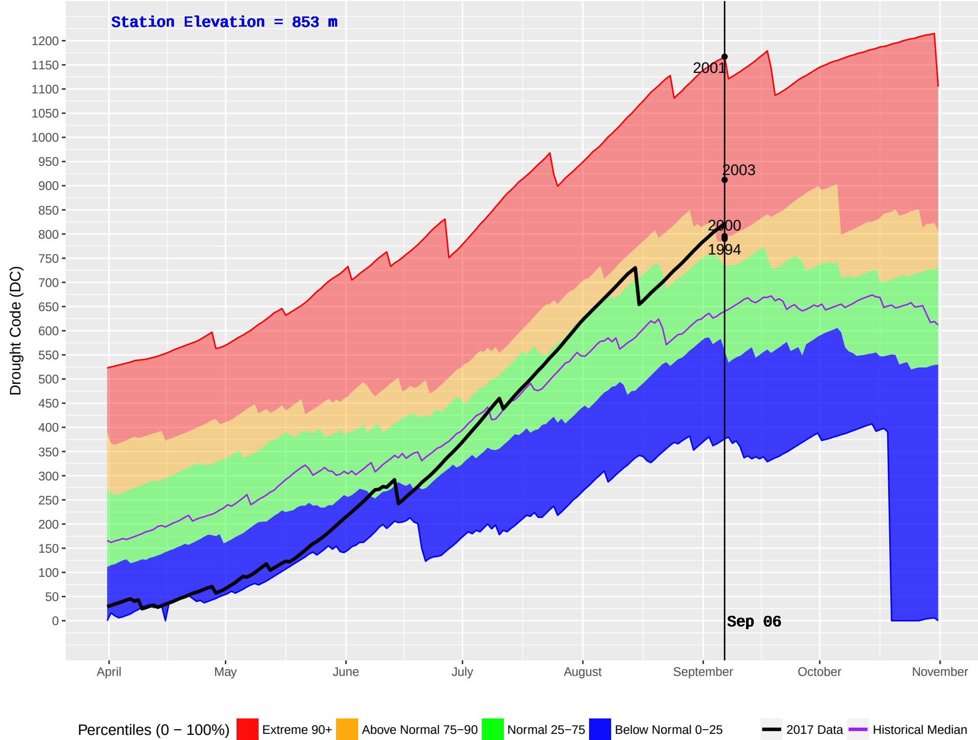
JOHNSON LAKE (419) : Historical (1986–2016) and Current (2017) Noon Drought Code (DC)
