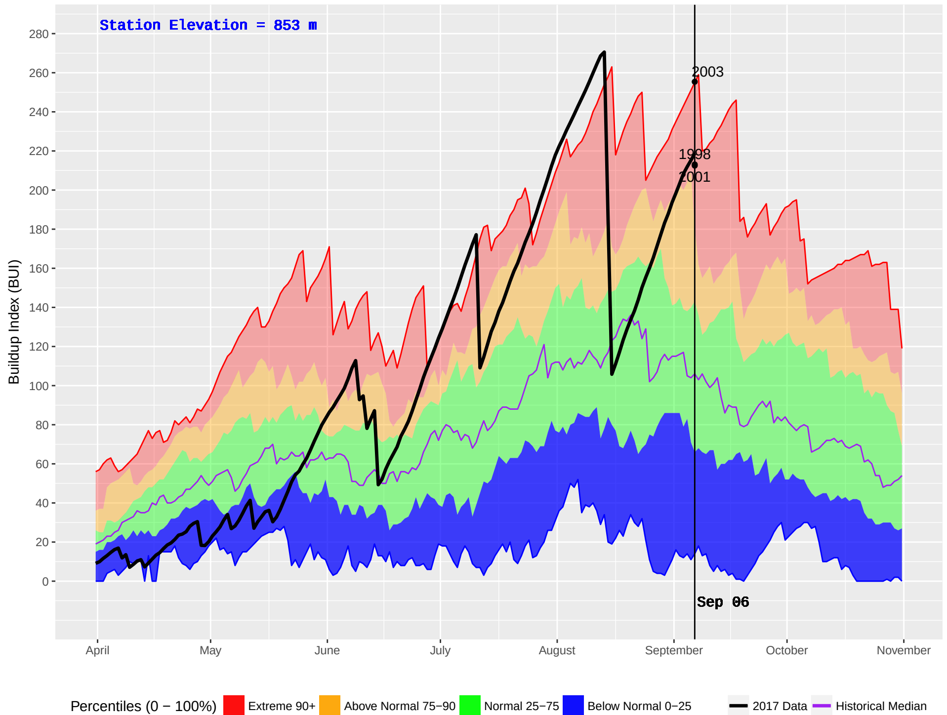
JOHNSON LAKE (419) : Historical (1986–2016) and Current (2017) Noon Buildup Index (BUI)
