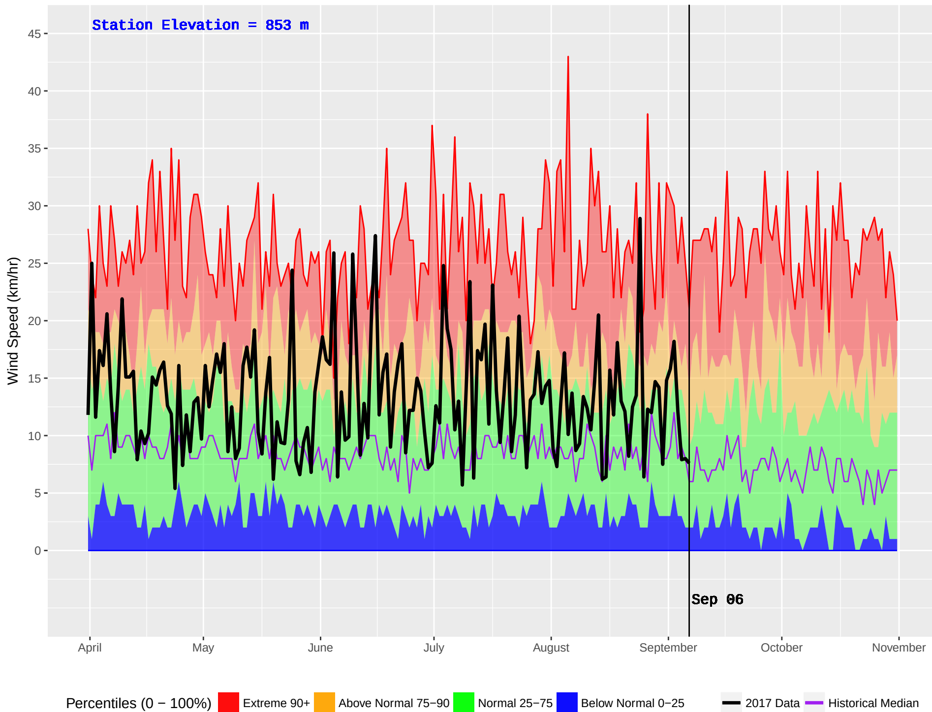
JOHNSON LAKE (419) : Historical (1986–2016) and Current (2017) Noon Wind Speed
